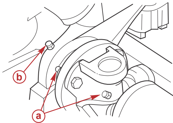
a - Driveshaft grease fittings b - Transom end grease fitting c - Engine end grease fitting
